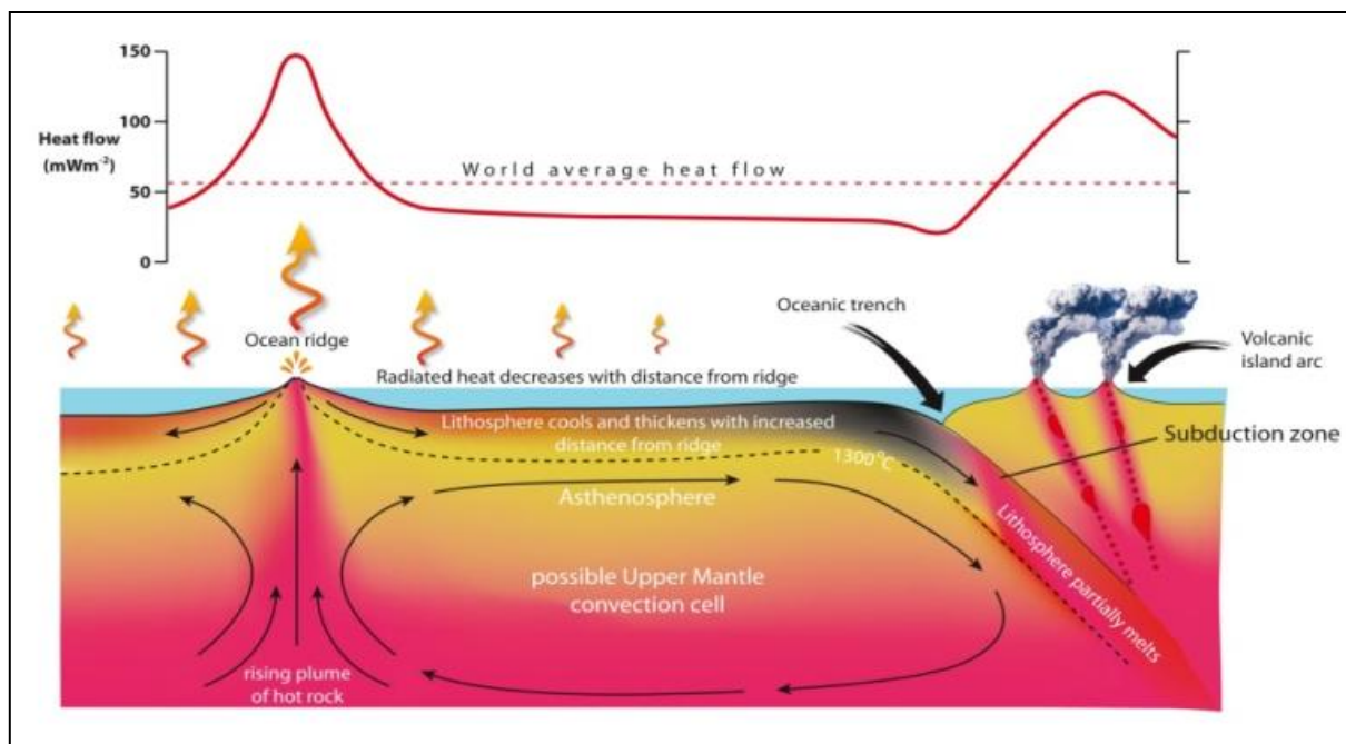
The pattern of heat flow out of the ocean floor and the upper part of the mantle and the crust.
