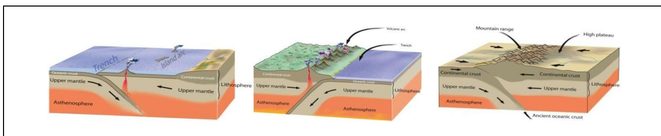
© Reproduced with the kind permission of the US Geological Survey, redrawn by ESEU
