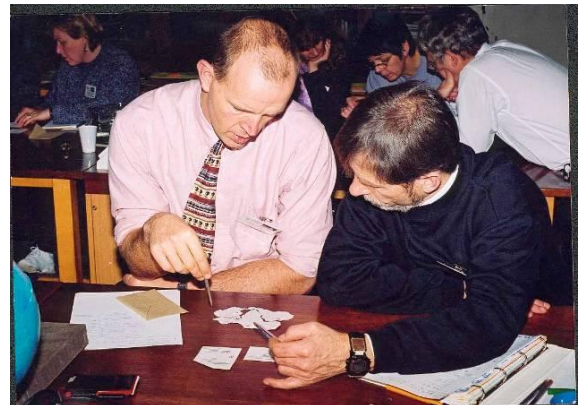
Debating the reconstruction of the super-continent 'Gondwanaland' © Peter Kennett
