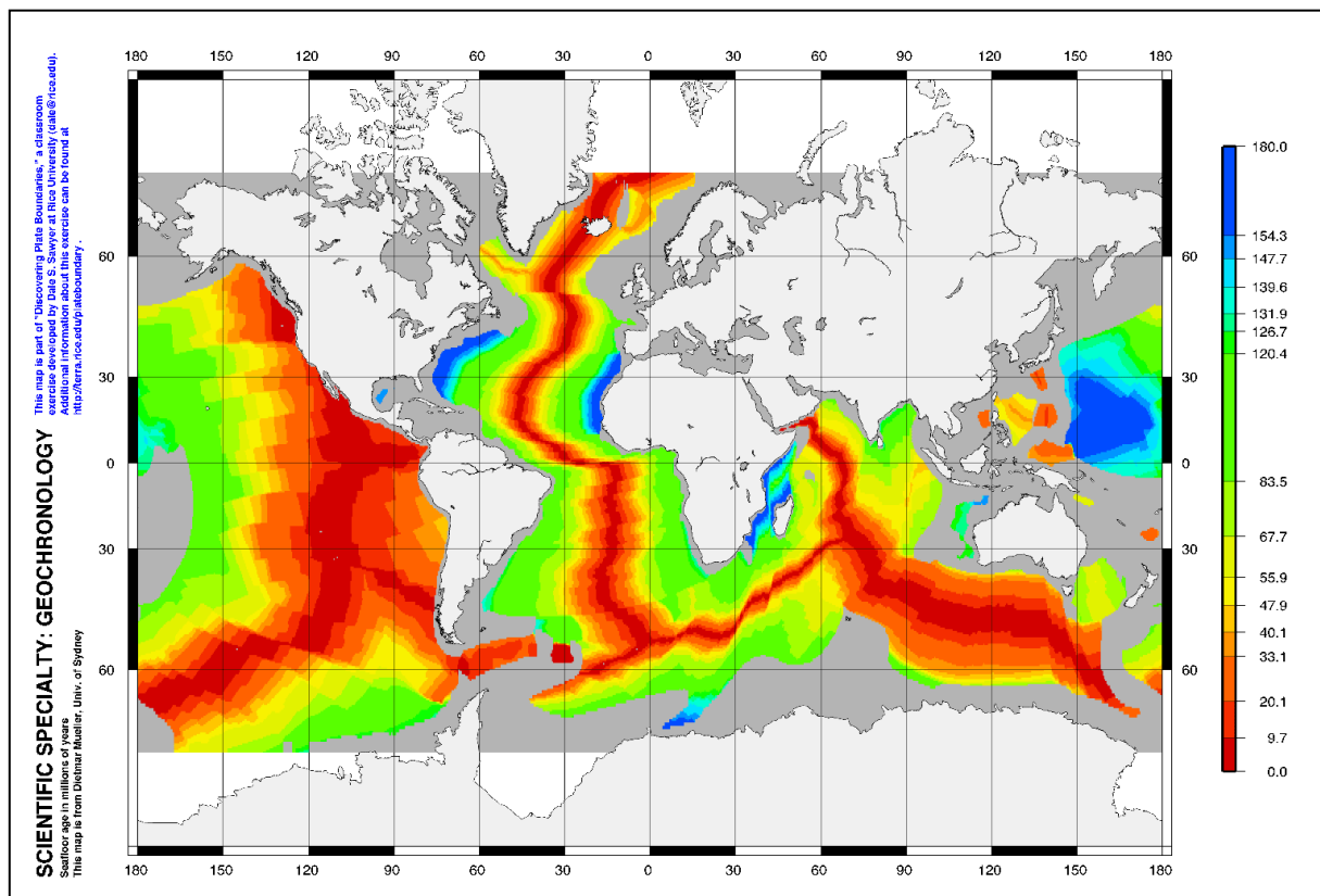
'The age of the sea floor'
