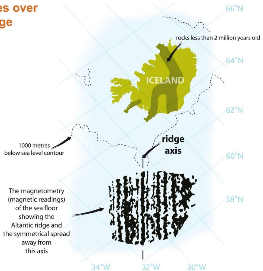
© Originally from Geoscience, redrawn by ESEU
