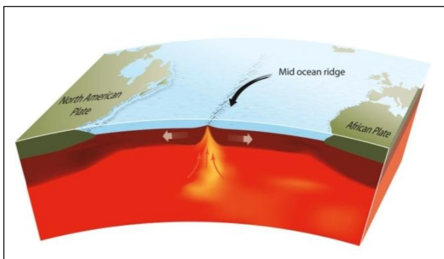
Mid ocean ridge © Press & Siever, redrawn by ESEU
