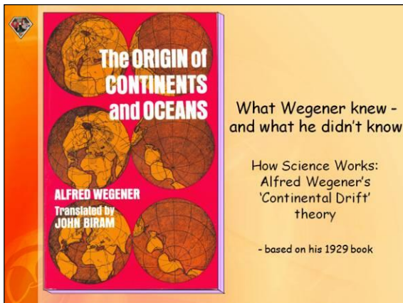
Screenshot from ESEU's PowerPoint 'What Wegener knew'
