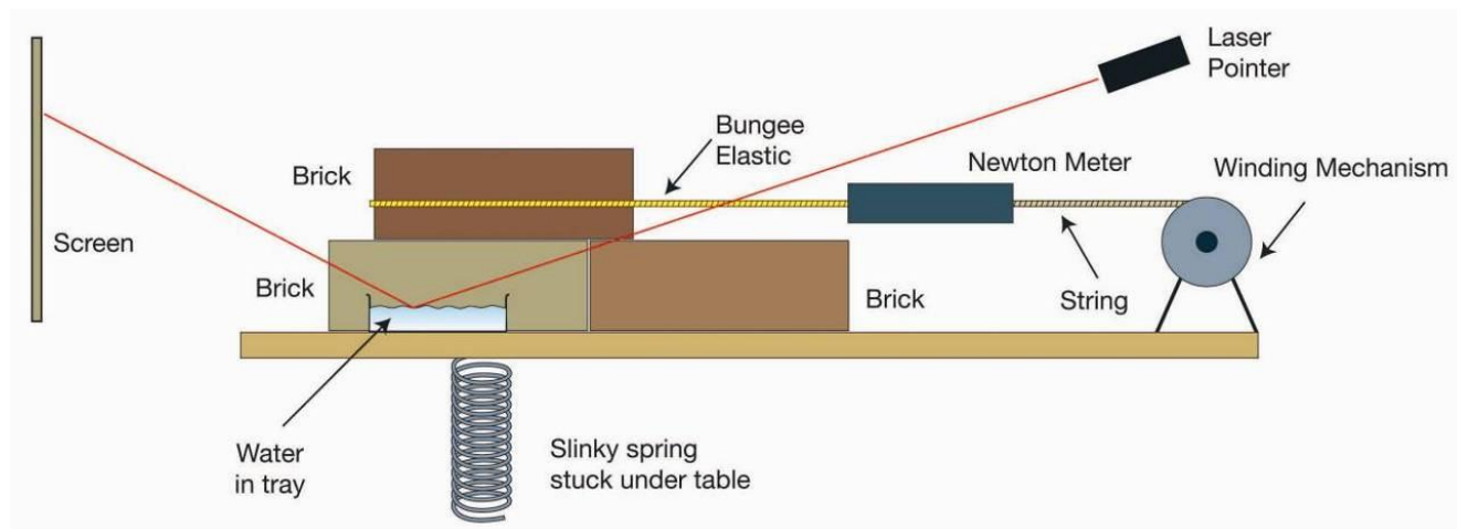
Diagram of apparatus for Brickquake © ESEU
