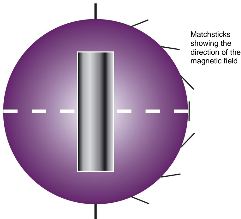
Model of the Earth's magnetic field © Chris King, ESEU
