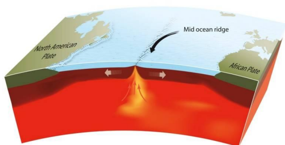
Mid ocean ridge © Press & Siever, redrawn by ESEU
