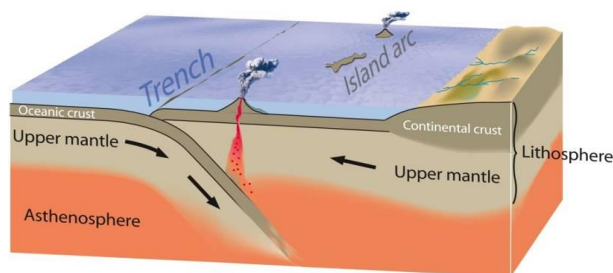
Ocean-ocean convergence. Reproduced with the kind permission of the U.S. Geological Survey, redrawn by ESEU
