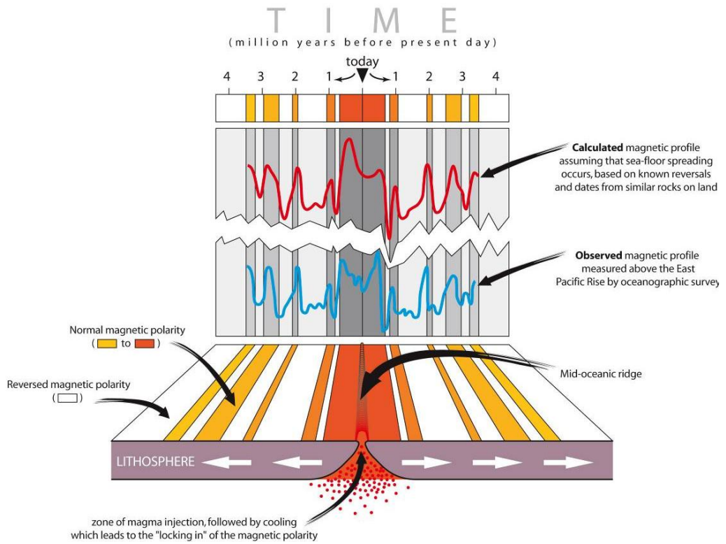
© originally from 'This Dynamic Earth: the Story of Plate Tectonics' by USGS, redrawn by ESEU
