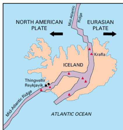
'Iceland, Mid-Atlantic Ridge' © USGS
