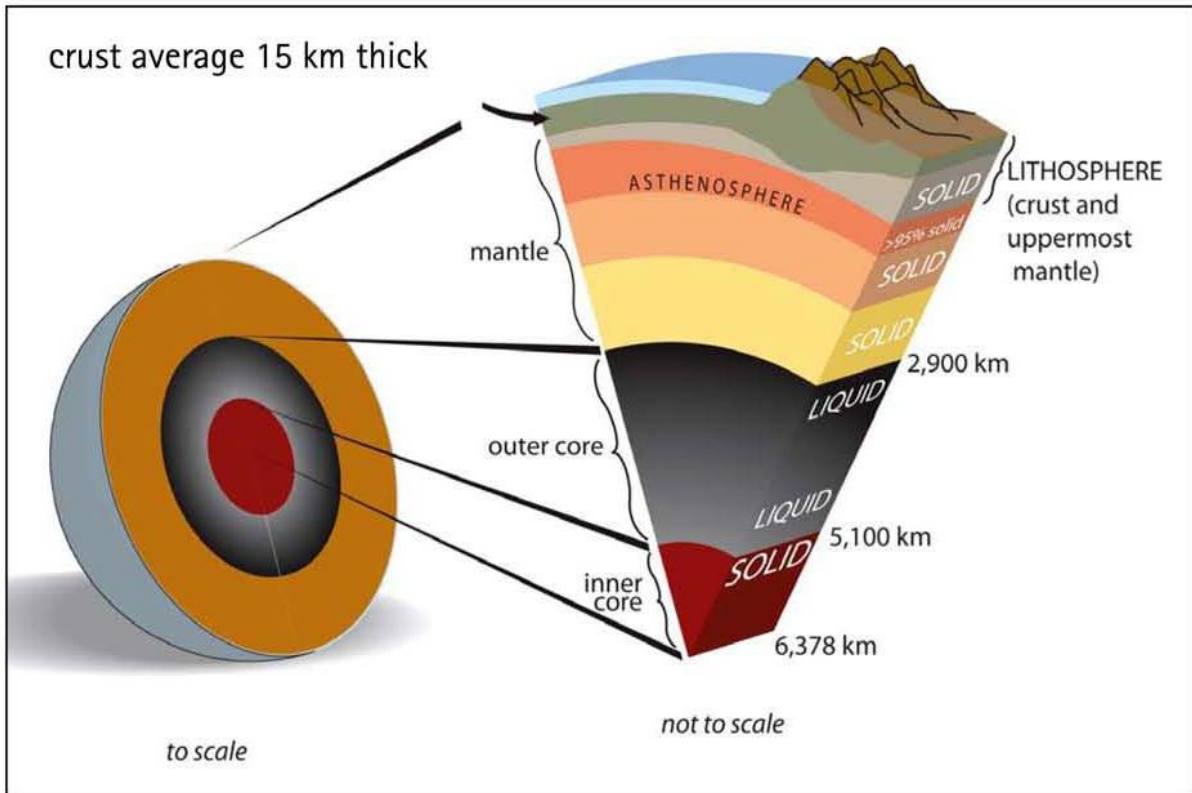
Diagram of the internal structure of the Earth. Reproduced with the kind permission of the U.S. Geological Survey, redrawn by ESEU
